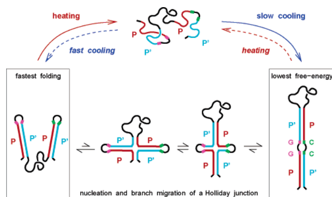
Figure 4. Driven and spontaneous transitions of the DNA switch. Heating and slow cooling (solid arrows) versus heating and fast cooling (dashed arrows) cycles drive the DNA switch back and forth between equilibrium, elongated conformation and out-of-equilibrium, contracted conformation through a denatured intermediate state in high ionic strength solution. Spontaneous relaxation operates on much longer time scales (beyond weeks at room temperature). The transition involves a nucleation step with simultaneous breaking of four base pairs in each hairpin helix and their rearrangement into an asymmetric Holliday junction, which is eventually resolved by spontaneous branch migration to form the lowest free-energy, elongated structure.
