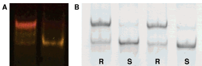
Figure 2. A DNA switch two operating modes. (A) Thermodynamics control: The DNA switch is equilibrated in a low ionic strength solution (1x TAE plus 0.1 M NaCl, left) or in a high ionic strength solution (1x TAE plus 1 M NaCl, right): the two bands correspond to the contracted conformation (high FRET, left) and the elongated conformation (low FRET, right). (B) Folding kinetics control: Electrophoresis separation (12% 19:1 acrylamide–bisacrylamide native gel) demonstrates three successive switchings between contracted (upper band) and elongated (lower band) conformations under heating/cooling cycles in constant high ionic strength solution (1x TAE plus 1 M NaCl). Rapid cooling (R lanes, >100 °C/ms, see Methods) leads to 80 \pm 3\% of fast folding, contracted conformations (ethidium bromide labeling), while moderate cooling rate (S lanes, <100 °C/s) leads to about 90% of lowest free-energy, elongated conformations.
